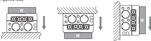
Fig. 1: Applied load
